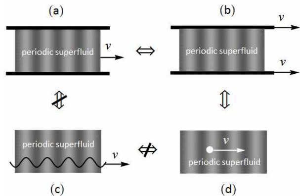
Fig. 5: In (a), (b), (d), the periodic superfluid and the lattice are locked in and move together with respect to the obstacle. In (c), the lattice is gradually accelerated to speed v . The reference frame is the lab. The scenario in (c) is not equivalent to the scenarios in (a), (b), (d) as there is relative motion between the lattice and the fluid in (c).
