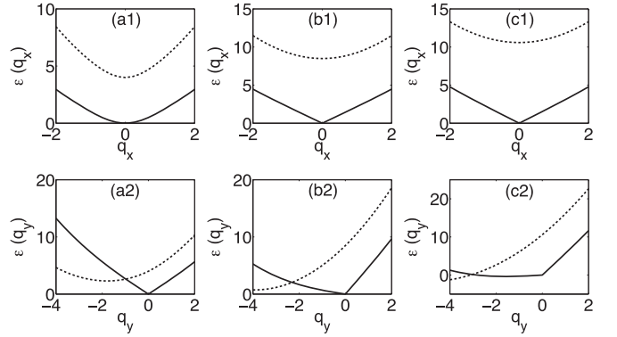
Fig. 3: Excitations along the x -axis (the first row) and y -axis (the second row) at different values of k . (a1), (a2): k = 1 ; (b1), (b2): k = 3 ; (c1), (c2): k = 4 . C_1 = 10 , C_2 = 4 , \gamma = 1 .
