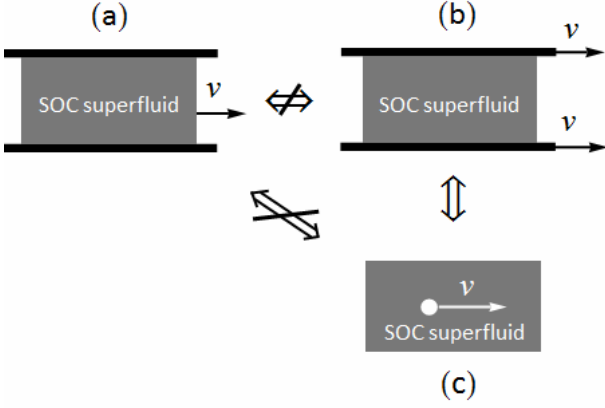
Fig. 1: (a) A superfluid with spin orbit-coupling moves while the tube is at rest. (b) The superfluid is dragged by a tube moving at speed v . (c) An impurity moves at v in the SOC superfluid. The reference frame is the lab. The two-way arrow indicates the equivalence between different scenarios and the arrow with a bar indicates the non-equivalence.
