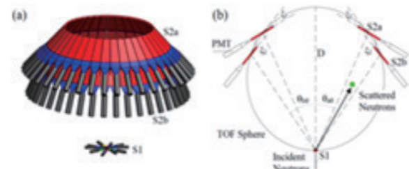
Fig. 2 3D representation of the TOFED spectrometer (a) and a vertical plane drawing (b) showing the positions of detectors on the sphere of diameter D . Each S2 ring consists of 40 detector units of scintillators and PM tubes with S1 being a five layered detector assembly.
