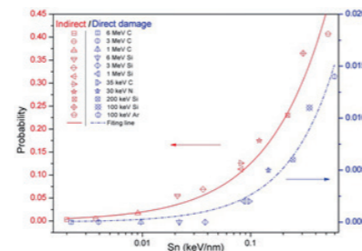
FIG. 4 MD simulations, and are plotted with respect to Sn in graphene and \text{Sn}_n in \text{SiO}_2 .
