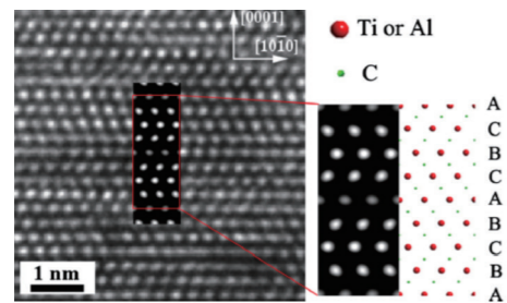
FIG. 1 HRTEM image of \text{Ti}_3\text{AlC}_2 irradiated at 5 \times 10^{16} \text{ cm}^{-2} ; the simulated phase contrast, shown in the inset, is superimposed on the experimental image.
