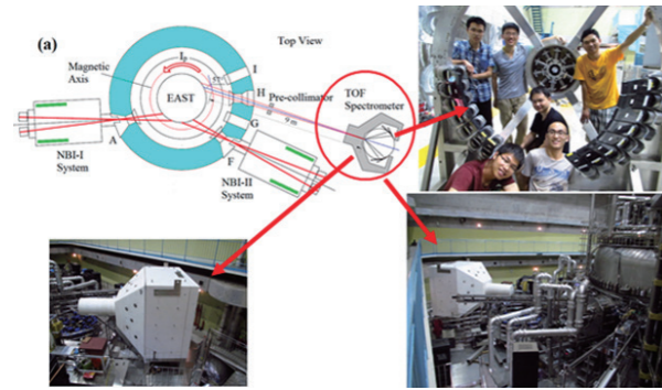
Fig. 1 The TOFED spectrometer installed in the EAST torus hall.
