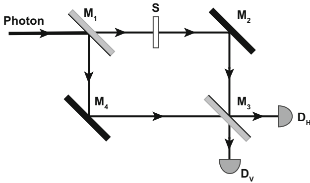
Fig. 1 Mach–Zehnder interferometer. M_1 and M_3 are half-silvered mirrors; M_2 and M_4 are reflective mirrors. S is some sample material that causes a phase shift to the photon’s wave function. D_H and D_V are two photon detectors. Note that M_1 and M_3 are not symmetric and their two sides are made of materials of different refractive indices
